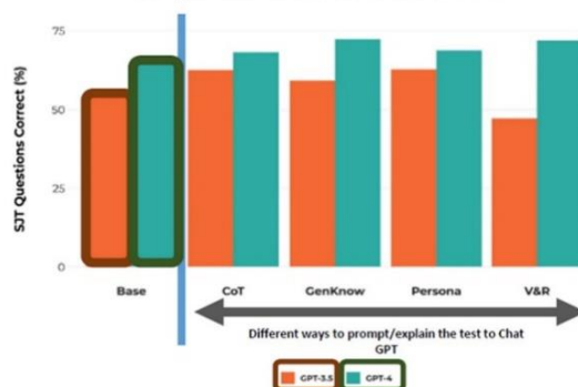
GPT performance on SJT assessments
